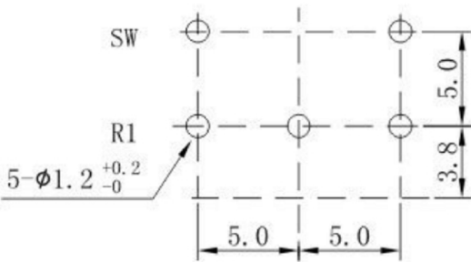
P. C. B MOUNTING HOLE DETAIL
