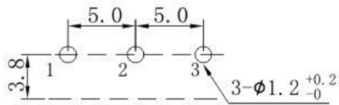
P. C. B MOUNTING HOLE DETAIL
