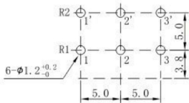
P. C. B MOUNTING HOLE DETAIL
