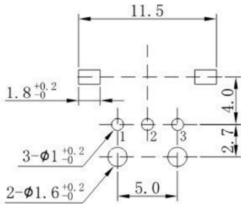
P. C. B MOUNTING HOLE DETAIL
