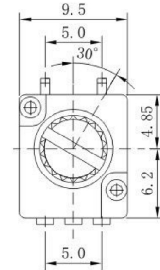
SHAFT SHOWN IN FULL C. C. W. POSITION
