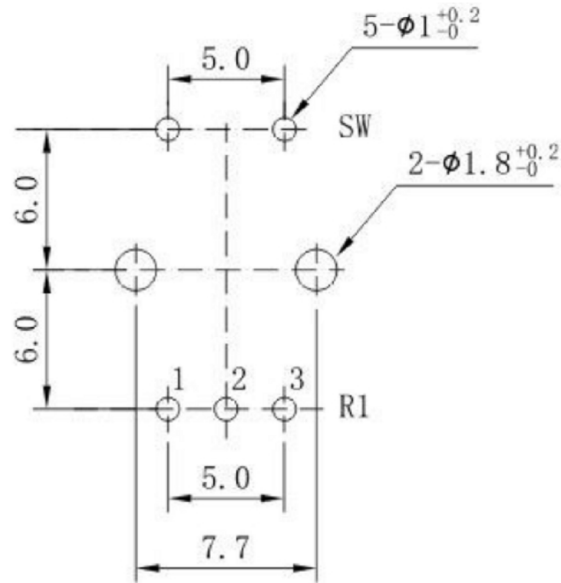
P. C. B MOUNTING HOLE DETAIL
