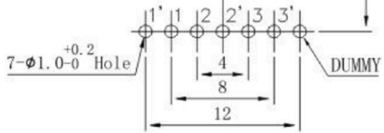
P. C. B MOUNTING HOLE DETAIL
