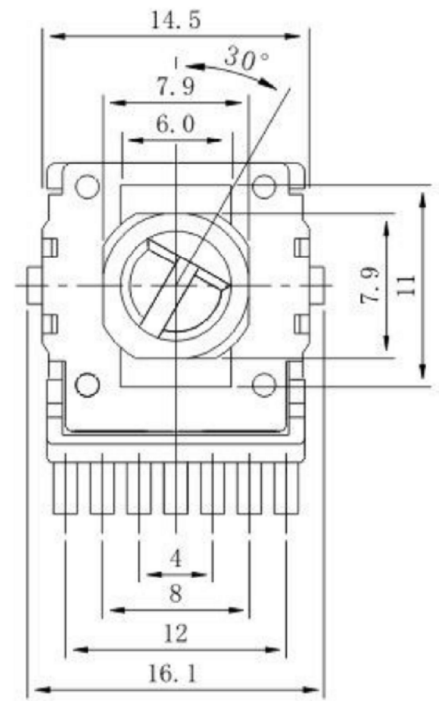
FULL C. C. W POSITION
