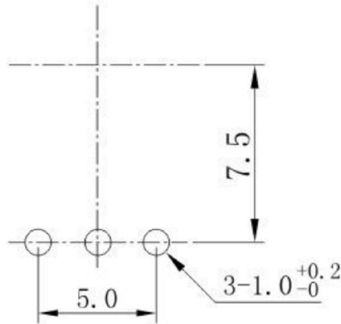
P. C. B MOUNTING HOLE DETAIL
