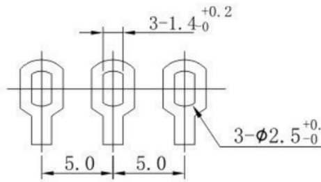
P. C. B MOUNTING HOLE DETAIL
