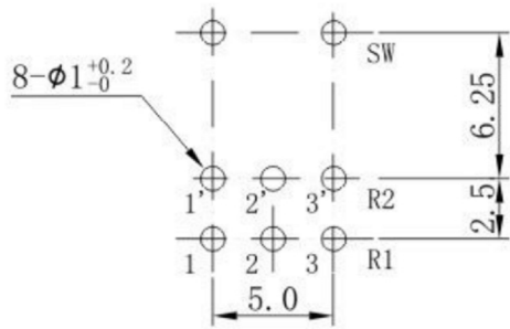
P. C. B MOUNTING HOLE DETAIL
