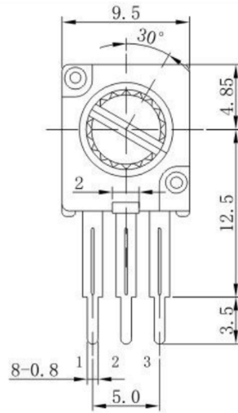
SHAFT SHOWN IN FULL C. C. W. POSITION
