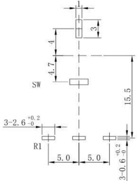
P. C. B MOUNTING HOLE DETAIL
