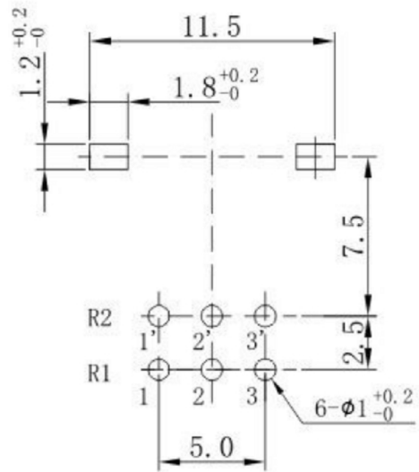
P. C. B MOUNTING HOLE DETAIL
