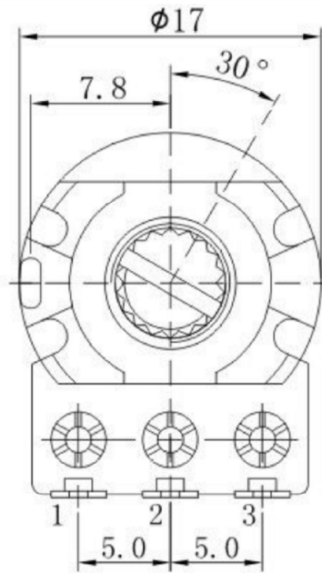
SHAFT SHOWN IN FULL C. C. W POSITION
