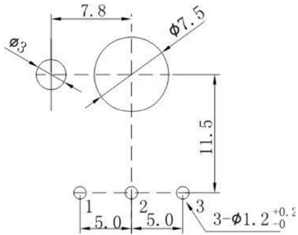
P. C. B MOUNTING HOLE DETAIL
