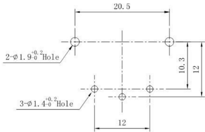
P. C. B MOUNTING HOLE DETAIL
