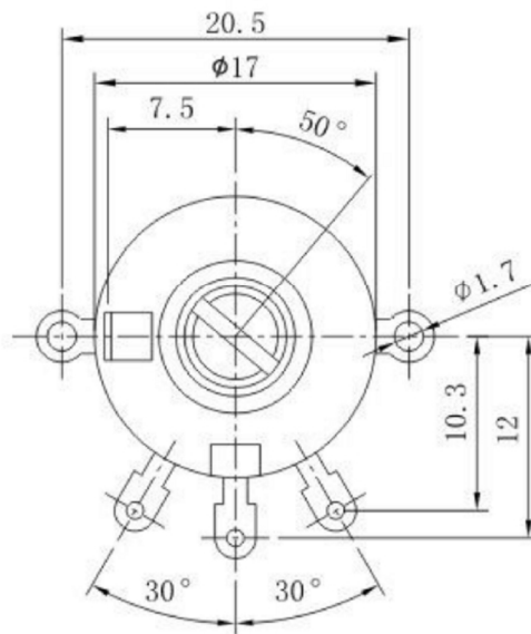
FULL C. C. W POSITION
