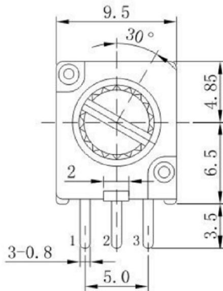
SHAFT SHOWN IN FULL C. C. W. POSTITION
