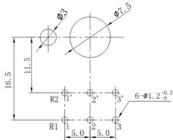
P. C. B MOUNTING HOLE DETAIL
