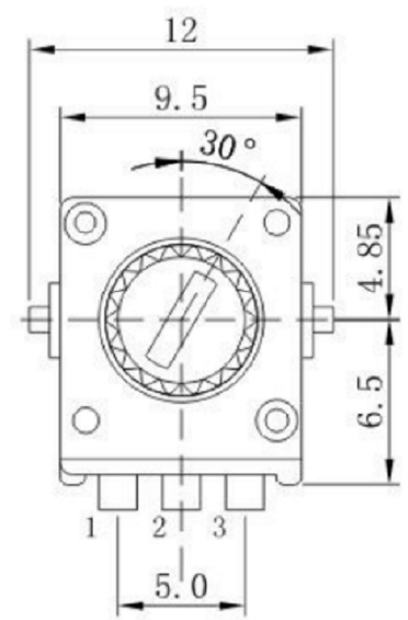
SHAFT SHOWN IN FULL C. C. W. POSITION
