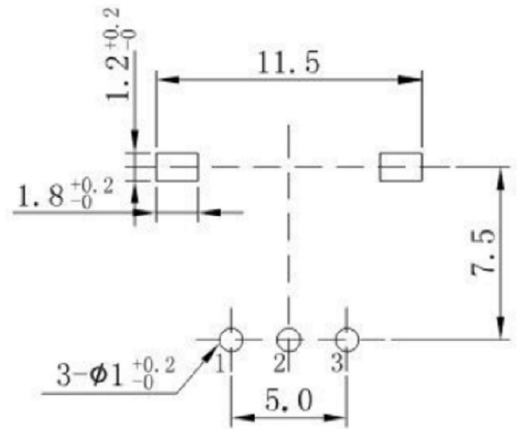
P. C. B MOUNTING HOLE DETAIL
