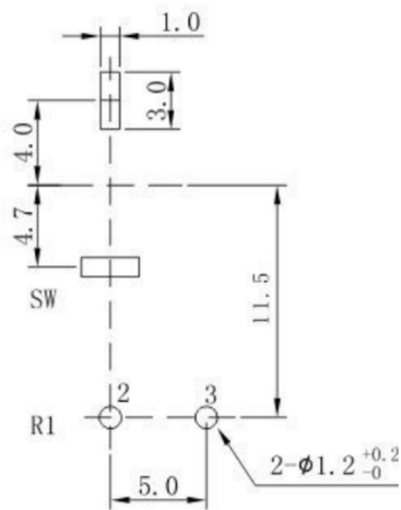
P. C. B MOUNTING HOLE DETAIL
