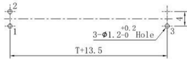
P. C. B MOUNTING HOLE DETAIL
