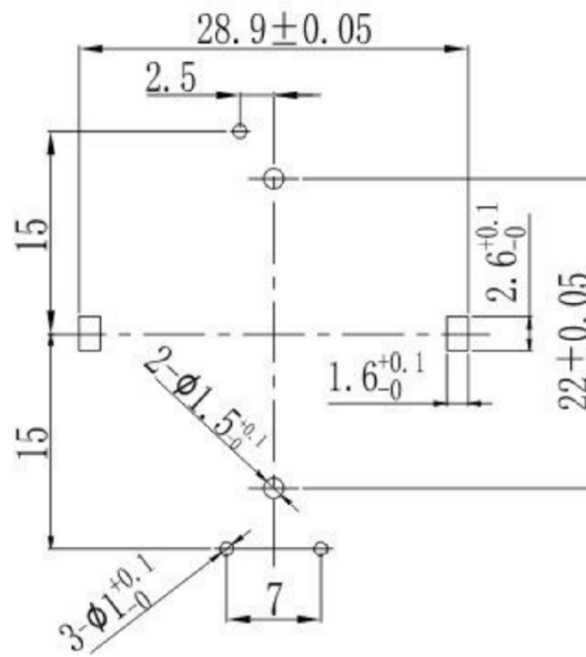
P. C. B MOUNTING HOLE DETAIL
