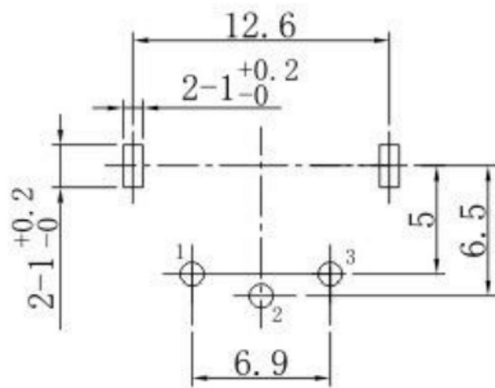
P. C. B MOUNTING HOLE DETAIL
