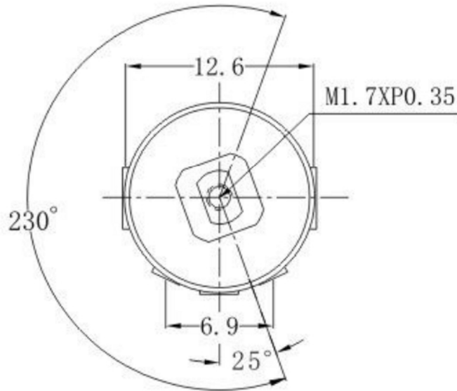
FULL C. C. W POSITION
