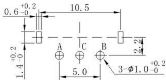
P. C. B MOUNTING HOLE DETAIL
