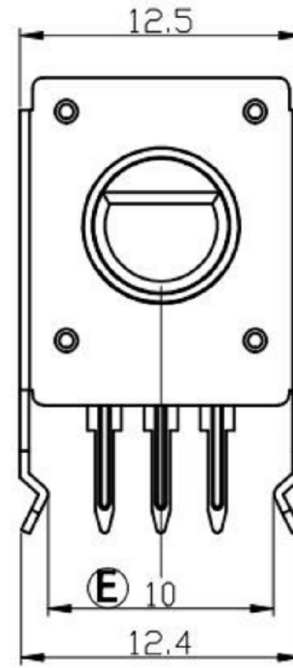
(SW01) ENCODER (SW02) PUSH ON SW CLICK Position
