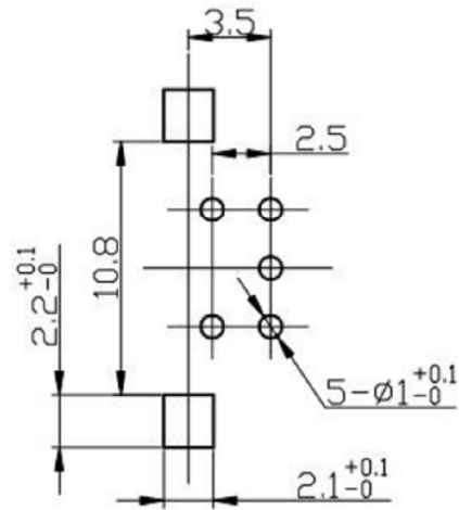
P.C.BOARD MOUNTING HOLE DIMENSIONS
