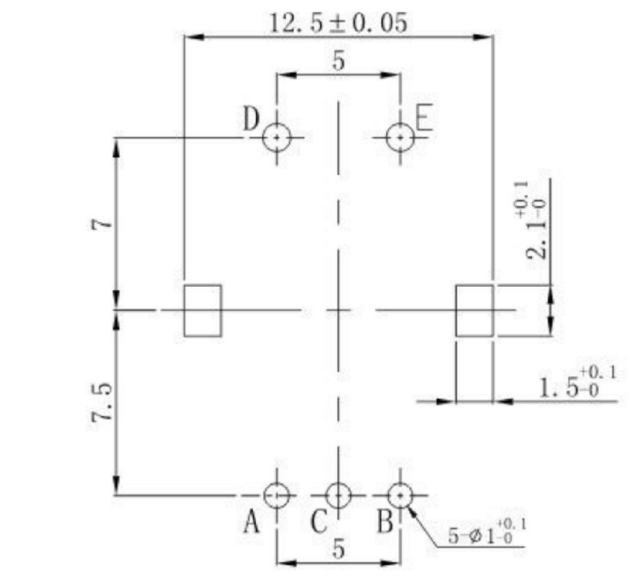
P. C. B MOUNTING HOLE DETAIL
