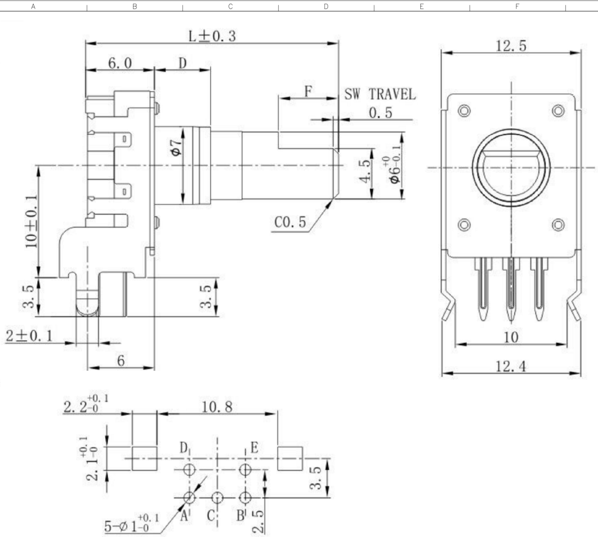
P. C. B MOUNTING HOLE DETAIL
