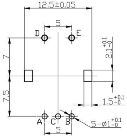
P.C.B MOUNTING HOLE DETAIL
