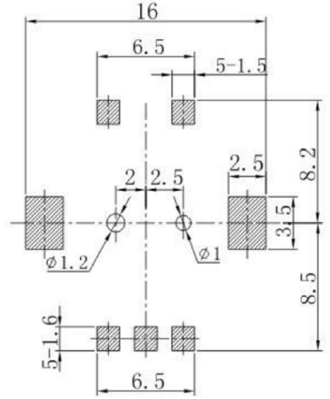
P.C.B MOUNTING HOLE DETAIL
