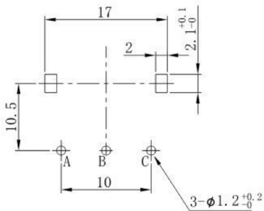
P. C. B MOUNTING HOLE DETAIL
