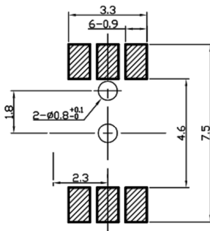
P.C.B.MOUNTING DETAIL
