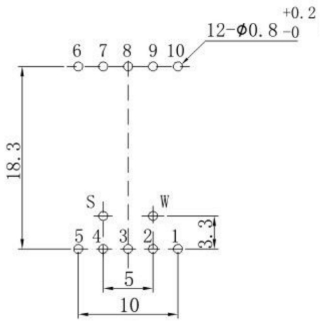
P. C. B MOUNTING HOLE DETAIL
