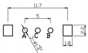
P. C. B MOUNTING HOLE DETAIL
