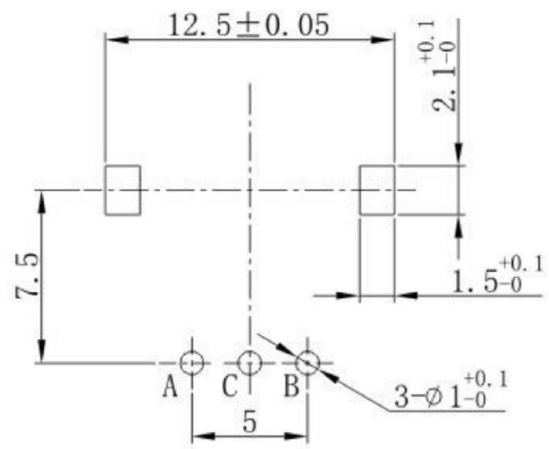
P. C. B MOUNTING HOLE DETAIL
