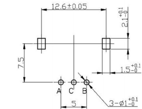
P.C.BOARD MOUNTING HOLE DIMENSIONS
