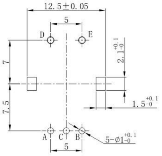
P. C. B MOUNTING HOLE DETAIL
