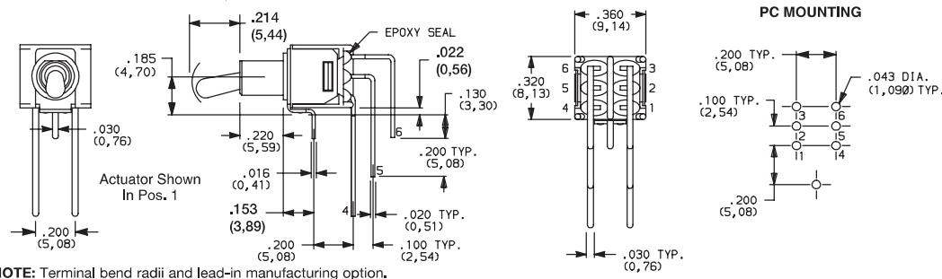
T201MH9AVBE Vertical Actuation DPDT
