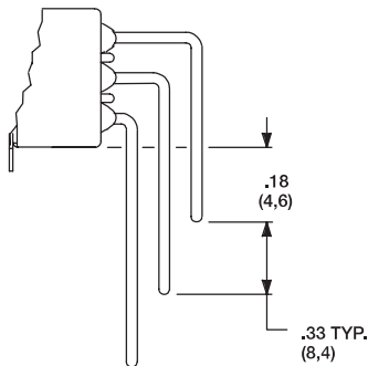
KSD-7301MD9ABE Horizontal Actuation 3PDT
