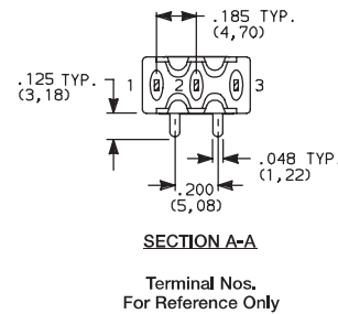
KSD-7101MD9ABE Horizontal Actuation SPDT
