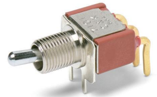
KSD-7101MHA2BE Horizontal Actuation SPDT
