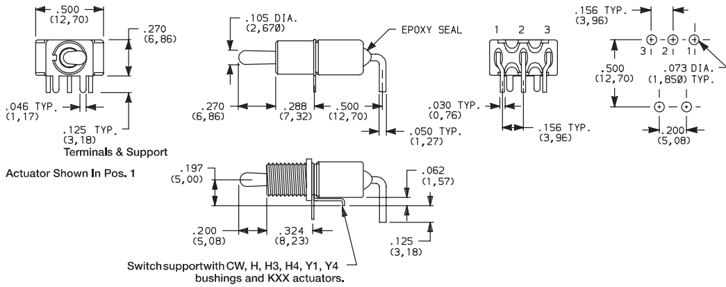
KSD-7101MHA2BE Horizontal Actuation SPDT
