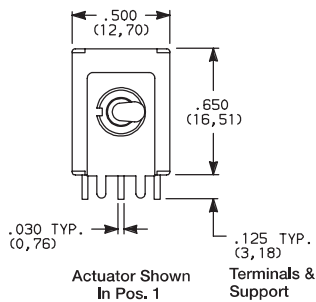
KSD-7301MD9ABE Horizontal Actuation 3PDT
