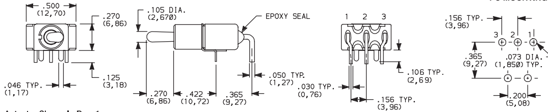
KSD-7101MD9A4BE Horizontal Actuation SPDT
