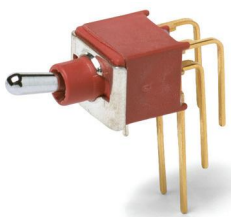
ET21MD1AVBE Vertical Actuation DPDT
