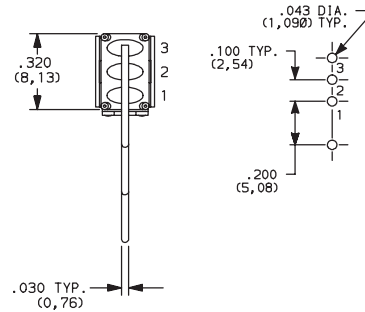
ET01SD1AV2BE Vertical Actuation SPDT
