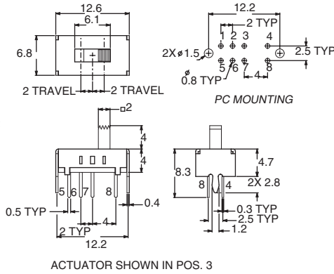
KSD-OS203011MS1QP1 DP3T
