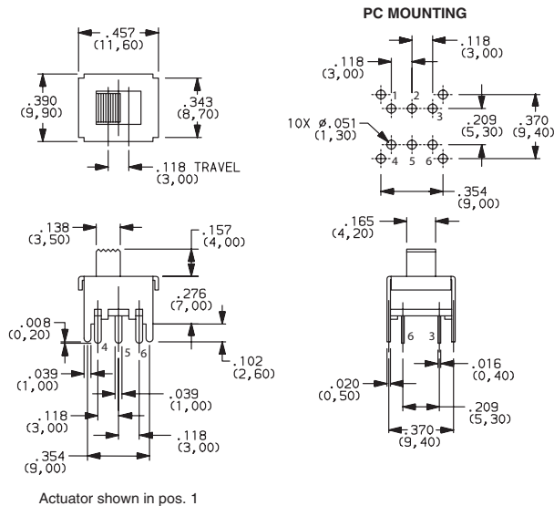
KSD-OS202013MT5QN1 DPDT
