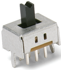
KSD-OS202011MS2QS1 DPDT
