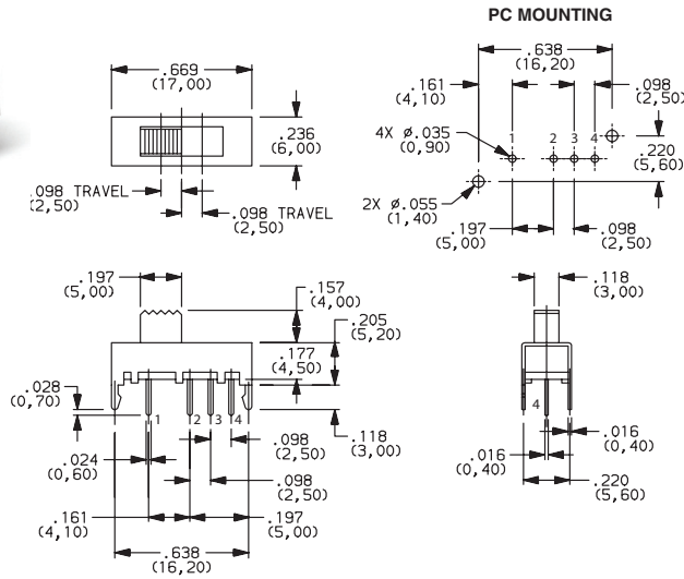
KSD-OS103012MU1QP1 SP3T
