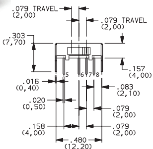
KSD-OS203011MA2QP1 DP3T
