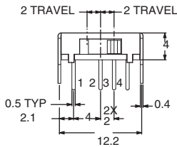
KSD-OS103011MA7QP1 SP3T
