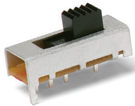
KSD-OS103012MU1QP1 SP3T
