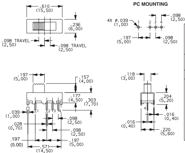
KSD-OS103012MU2QP1 SP3T
