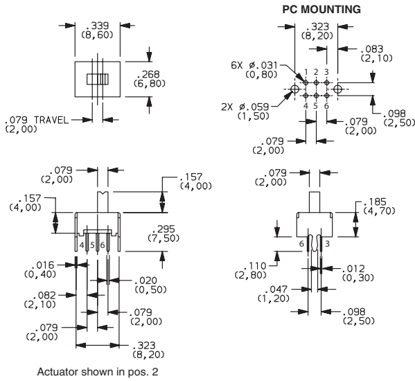
KSD-OS202011MS2QS1 DPDT
