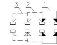
NON-SHORTING SCHEMATIC
