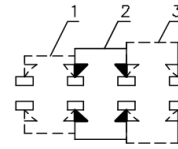
NON-SHORTING SCHEMATIC
