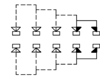
(NON-SHORTING) SCHEMATIC
