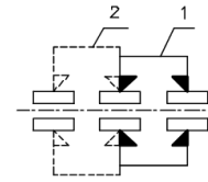
NON-SHORTING SCHEMATIC
