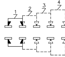
NON-SHORTING SCHEMATIC
