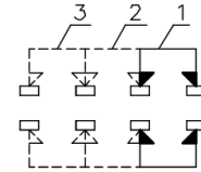
NON-SHORTING SCHEMATIC
