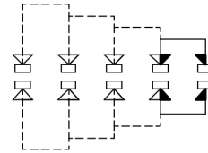
NON-SHORTING SCHEMATIC
