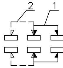
SHORTING SCHEMATIC
