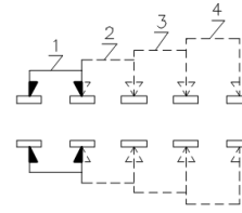
NON-SHORTING SCHEMATIC
