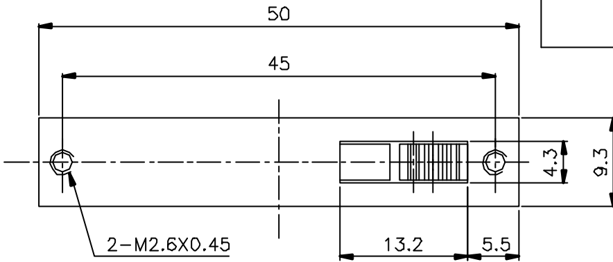
SCHEMATIC
