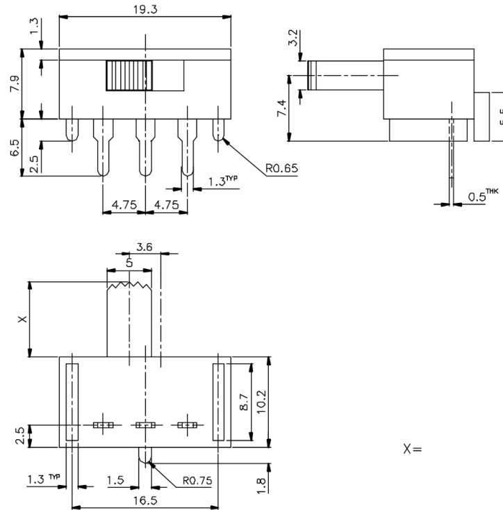
SCHEMATIC
