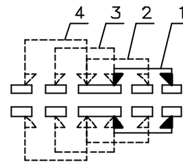
NON-SHORTING SCHEMATIC
