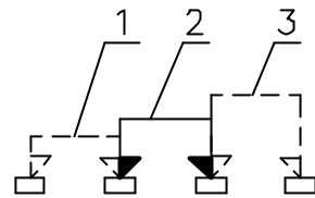
NON-SHORTING SCHEMATIC
